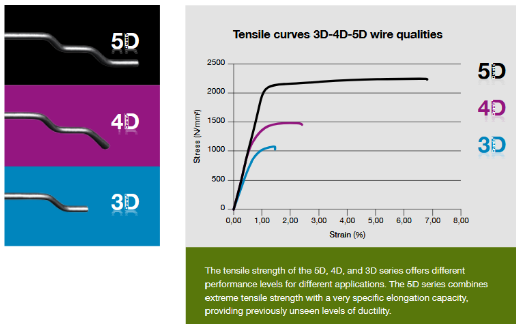
Figure 2. The tensile strength of Dramix® product series.
