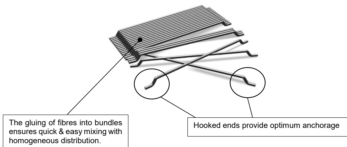
Figure 1. Technical concept of the Dramix® 3D fibre.
